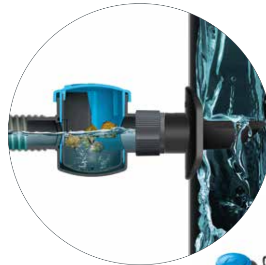
Filter with valve
